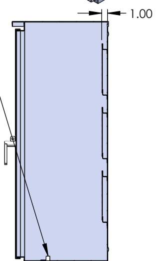
SIDE VIEW SECTIONED
